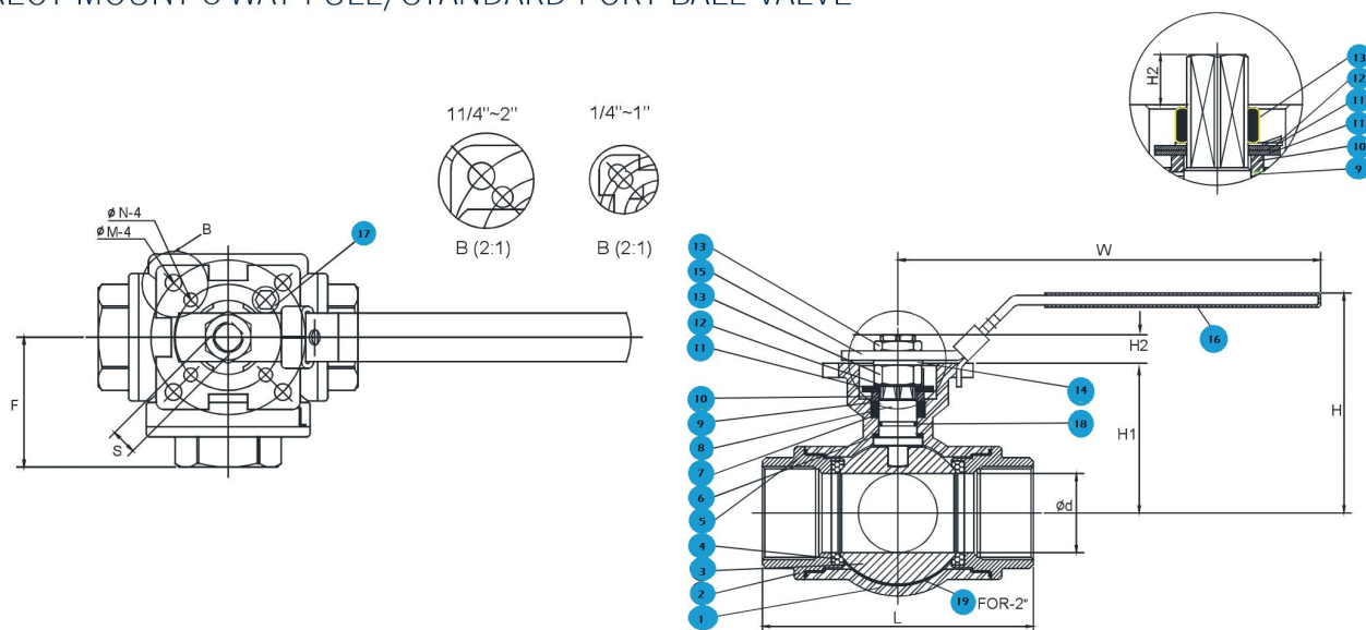
Dimensions - Standard Port (mm):
